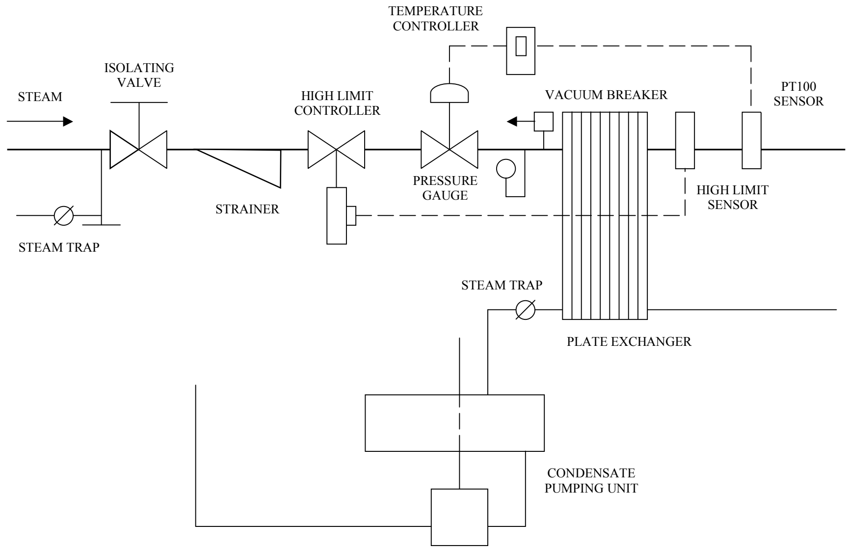
RECOMMENDED STEAM PLATE EXCHANGER LAYOUT
